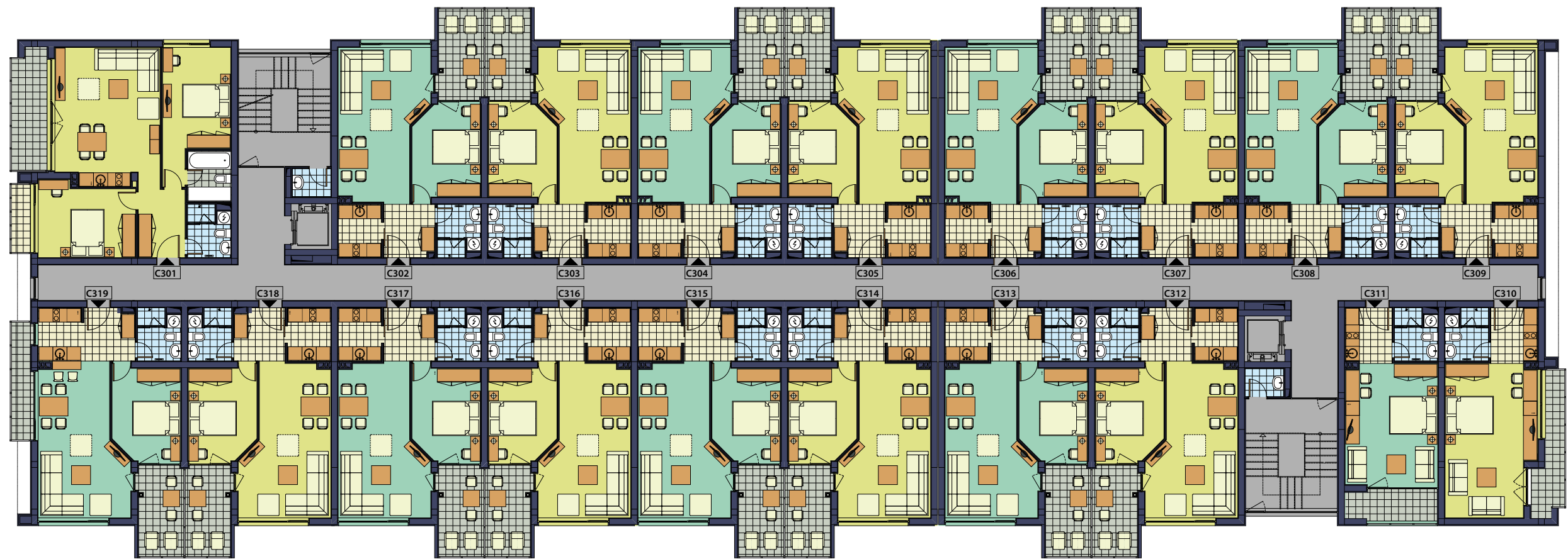
Building C, Third floor (+5.80)
