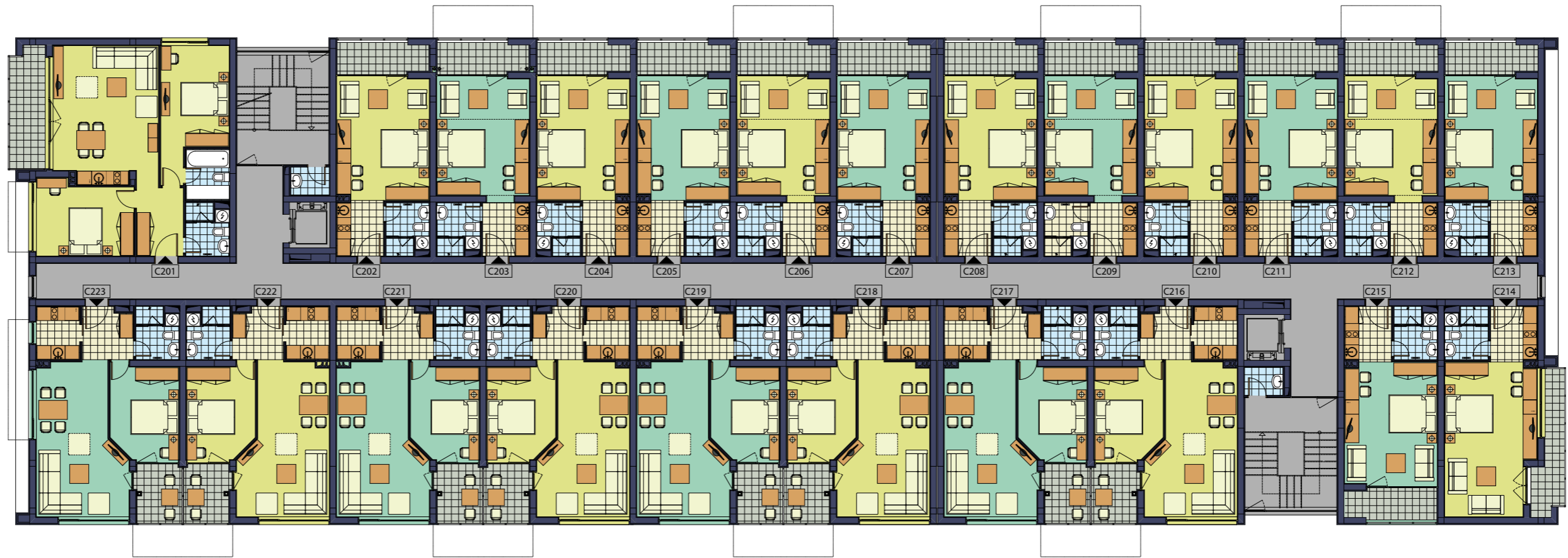
Building C, Second floor (+2.90)
