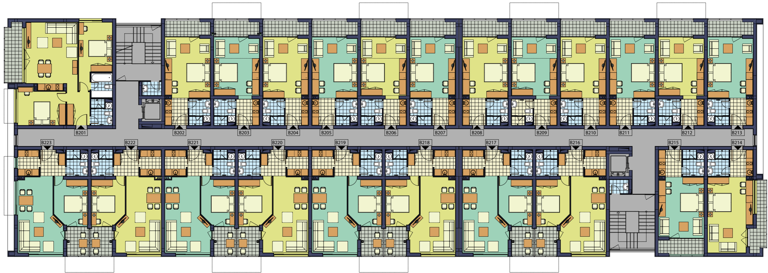
Building B, Second floor (+2.90)
