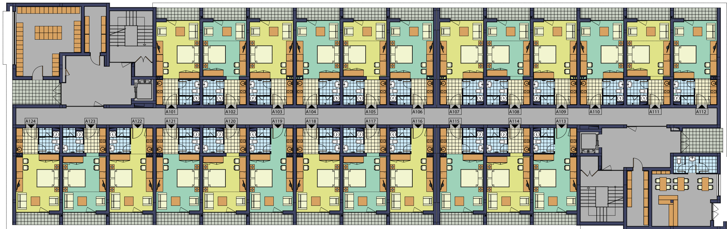
Building A, First floor (±0.00)
