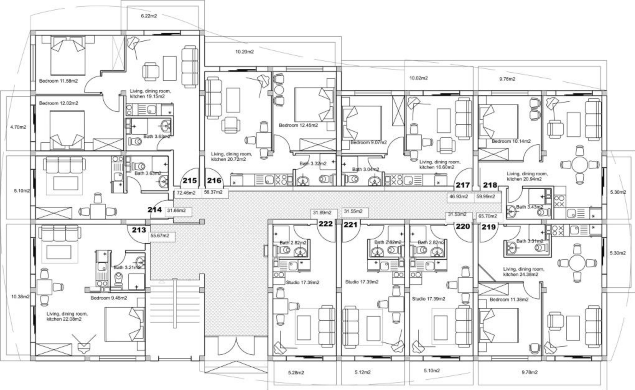
GROUND FLOOR HOUSE VII(7)
